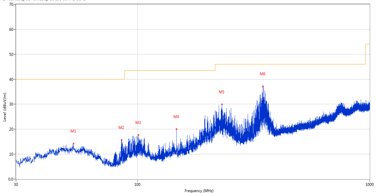
RE Test case_FCC Part 15C_FCC 15C 30MHz-1GHz
