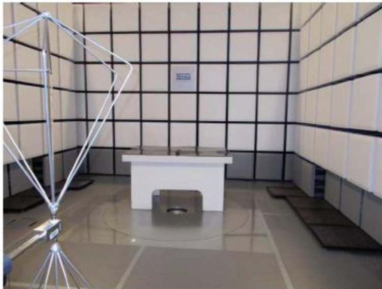
Figure 3: Radiated emission test 30 MHz – 200 MHz (without charger)
