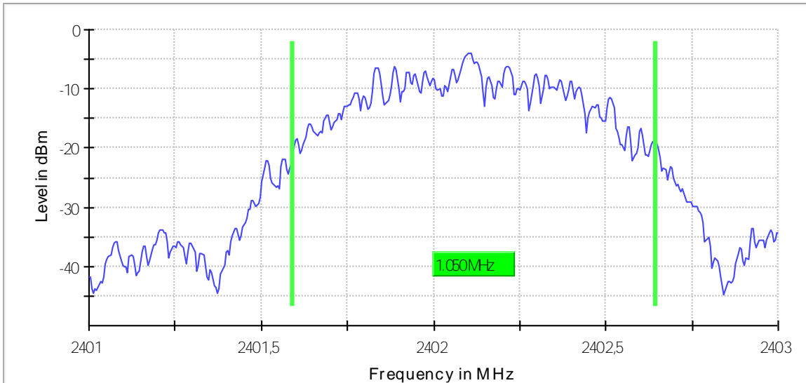
99 % Bandwidth
