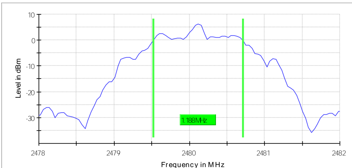
6dB Bandwidth
