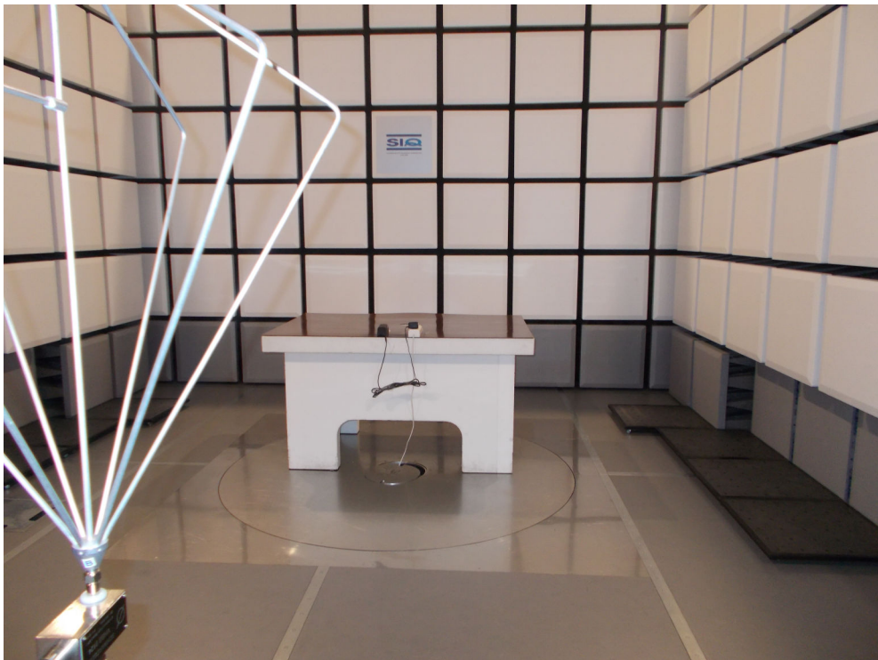
Figure 4: Radiated emission test – charging from AC/DC power supply
