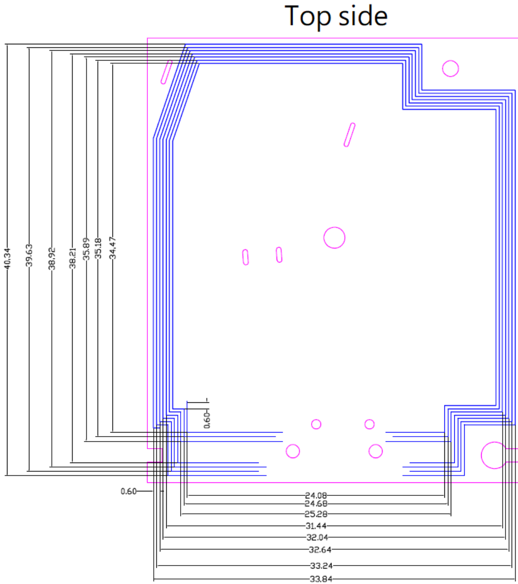
Figure1. Antenna patterns
