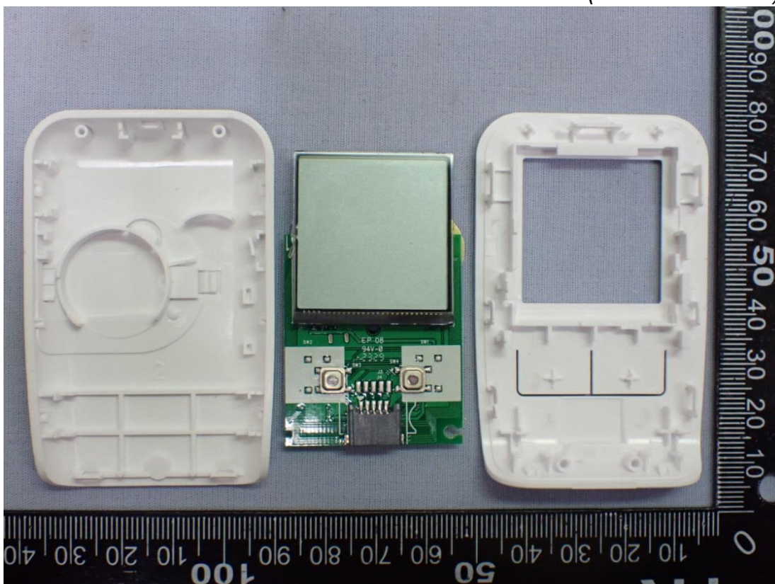
Internal View (Removed Cover)
