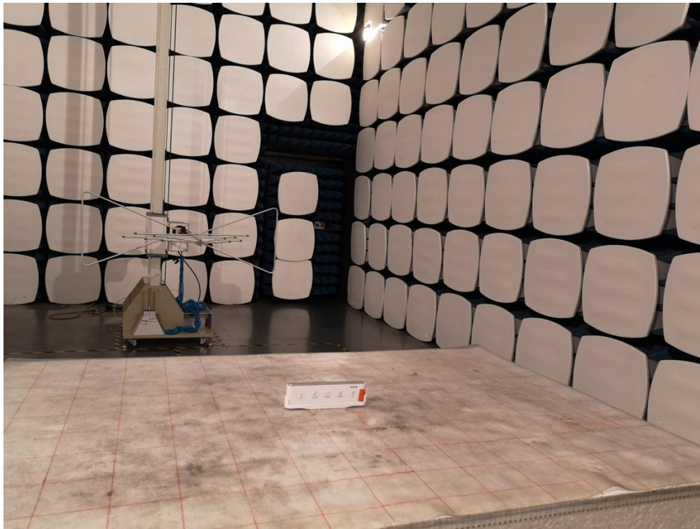
RC10-03 Radiated Emission Below 1GHz
