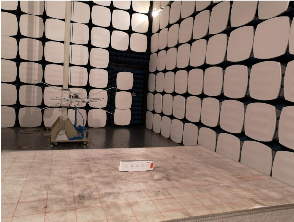
RC10-02 Radiated Emission Below 1GHz
