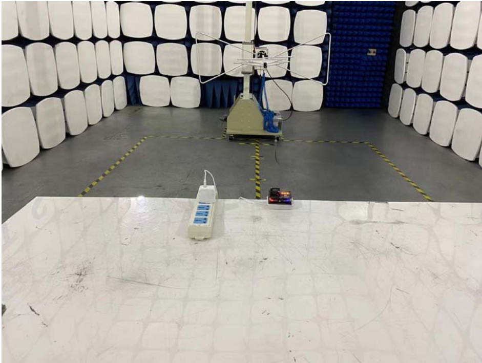
Radiated Emission Photo 2
