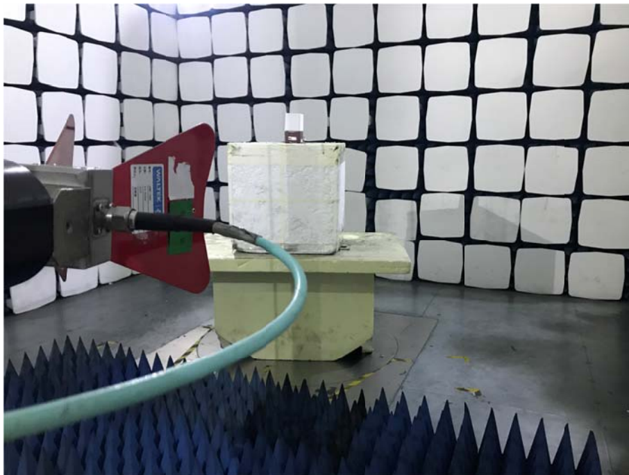
Radiation Emission Test Setup (1000MHz to 18GHz)
