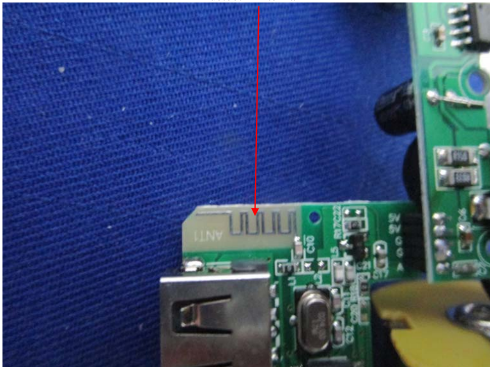
Bluetooth Antenna
