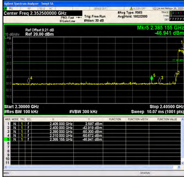
Channel 0 / 2402 MHz – Hopping
