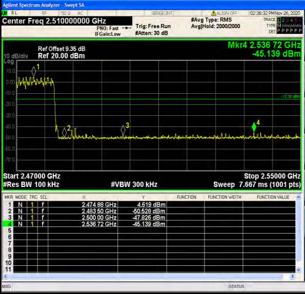
Channel 78 / 2480 MHz – Hopping
