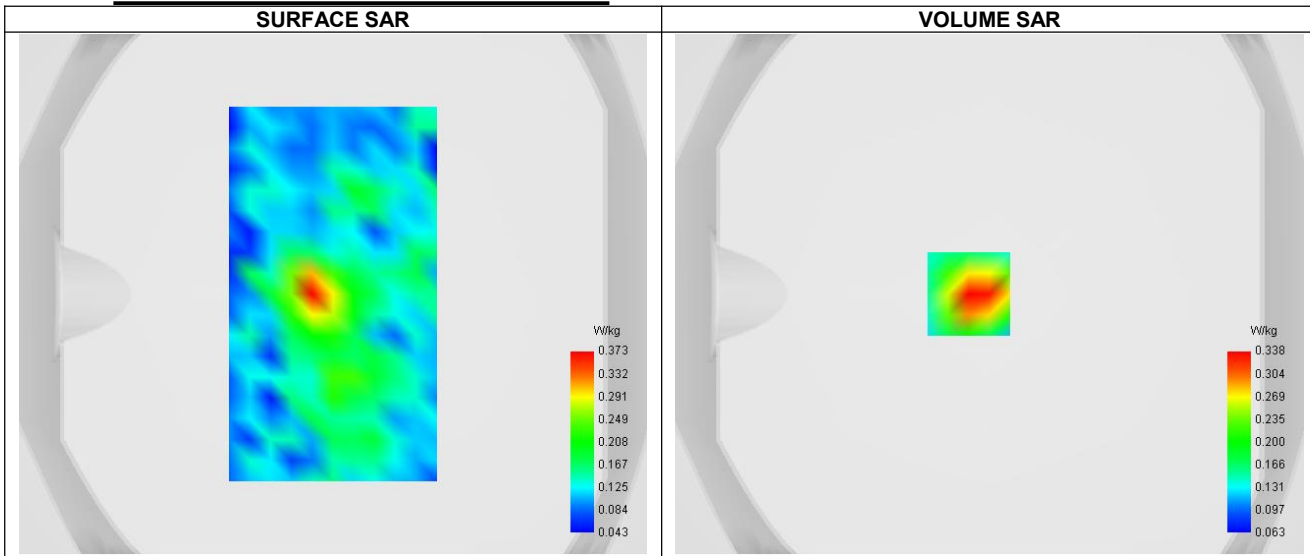
Maximum location: X=-8.00, Y=0.00 ; SAR Peak: 0.49 W/kg
