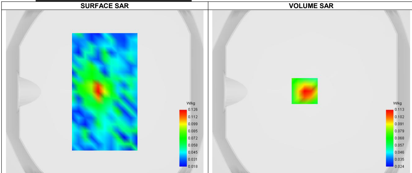
Maximum location: X=-8.00, Y=1.00 ; SAR Peak: 0.17 W/kg
