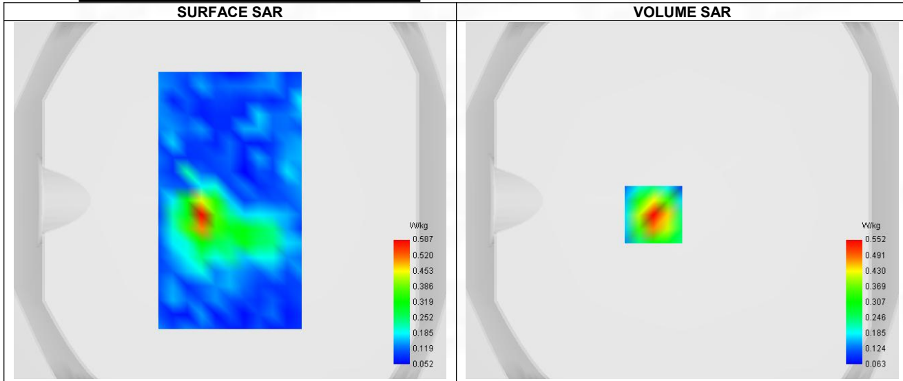
Maximum location: X=-16.00, Y=-8.00 ; SAR Peak: 0.86 W/kg
