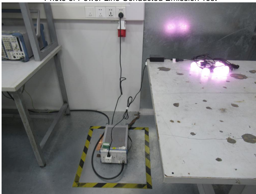
FCC ID: 2AQA6-H7022 Photo of Power Line Conducted Emission Test
