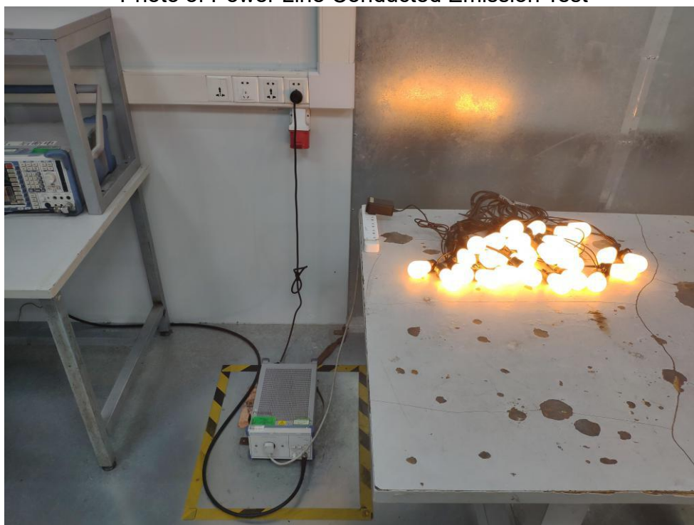
FCC ID: 2AQA6-H7011 Photo of Power Line Conducted Emission Test
