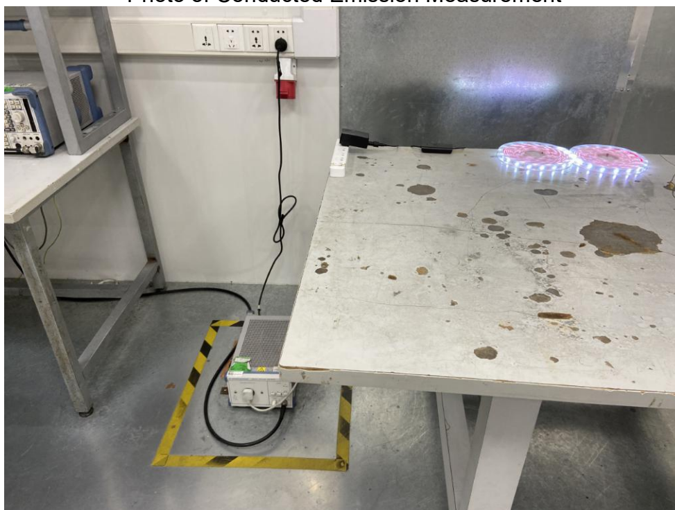
FCC ID: 2AQA6-H6170 Photo of Conducted Emission Measurement
