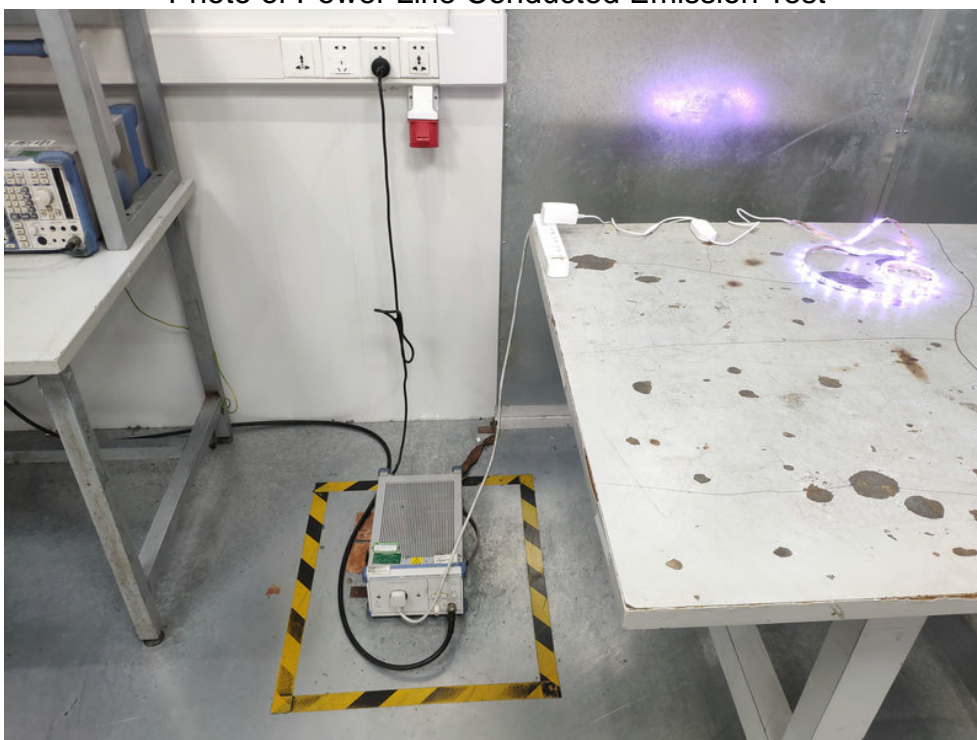
FCC ID: 2AQA6-H6141 Photo of Power Line Conducted Emission Test
