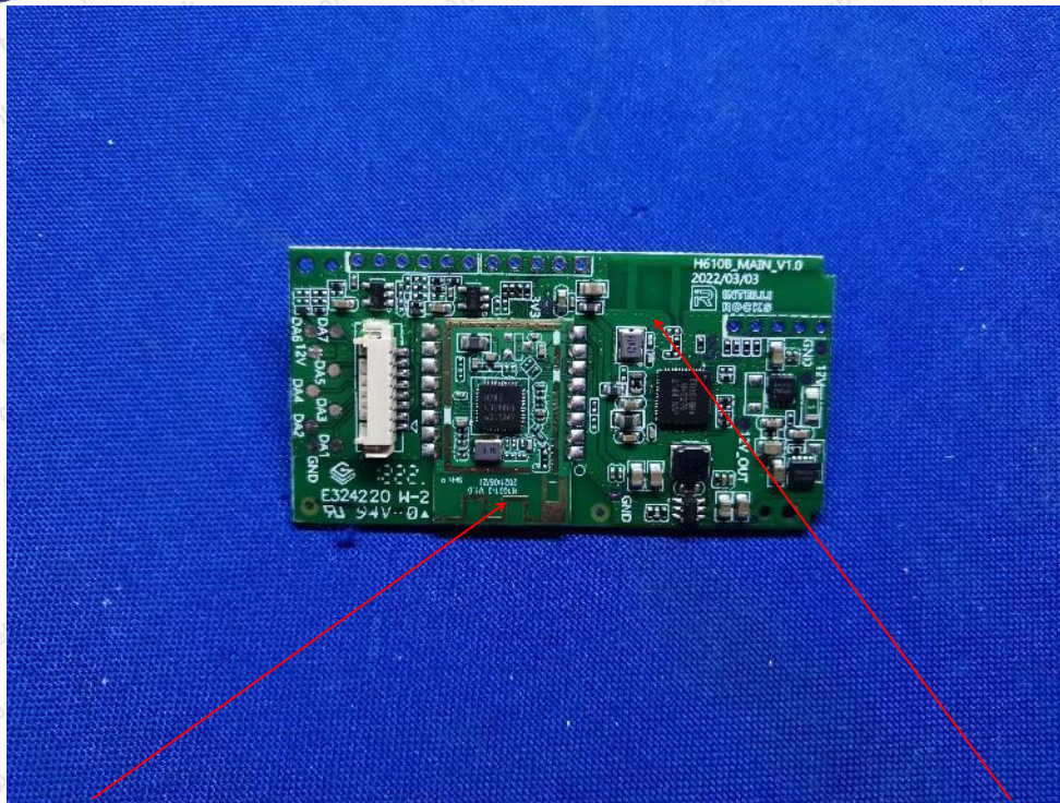
WIFI ANT
