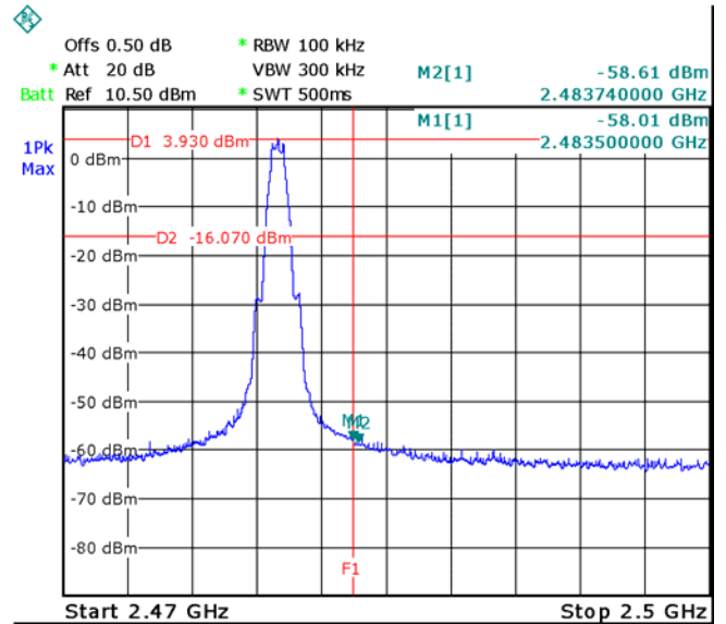
BLE: Band edge-right side
