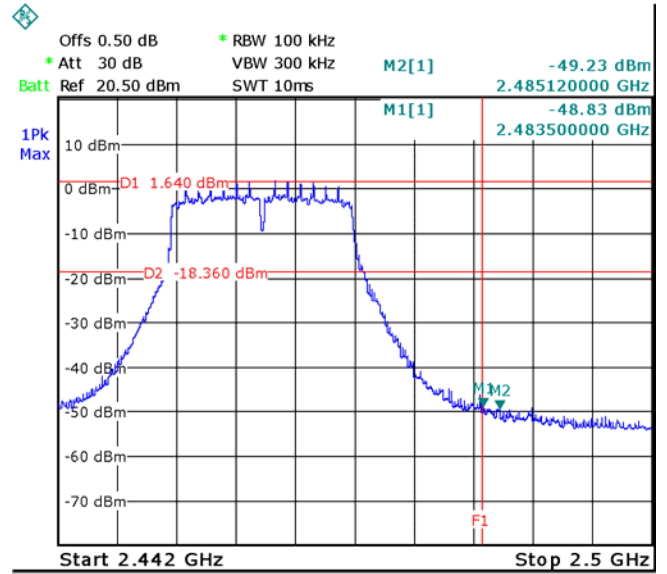
TX 11n HT20: Band edge-right side
