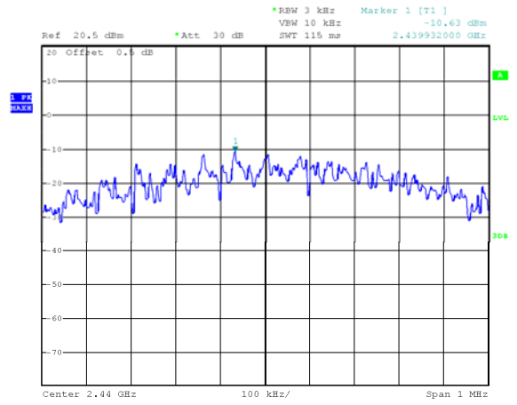
Mode: TX GFSK channel 19
