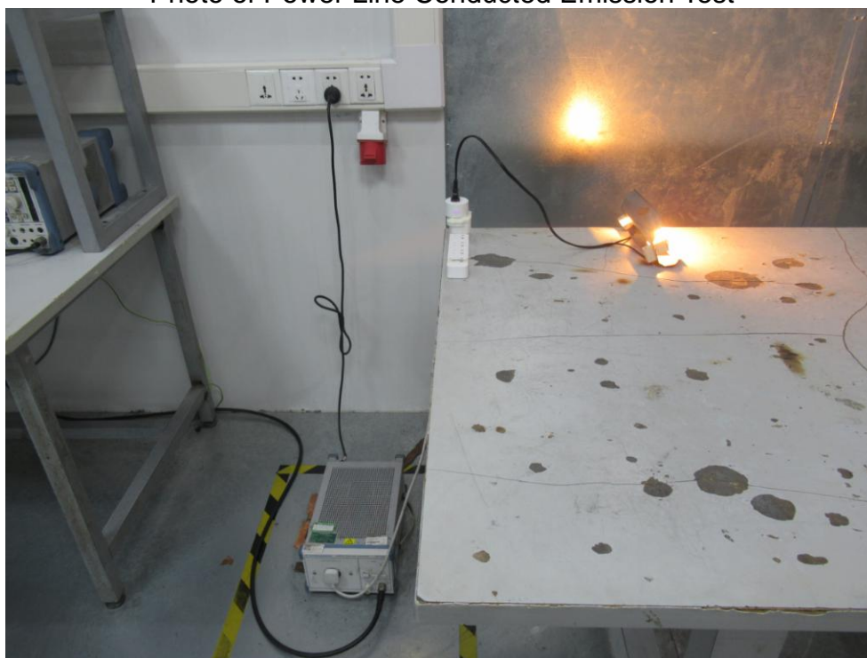
FCC ID: 2AQA6-H5081 Photo of Power Line Conducted Emission Test
