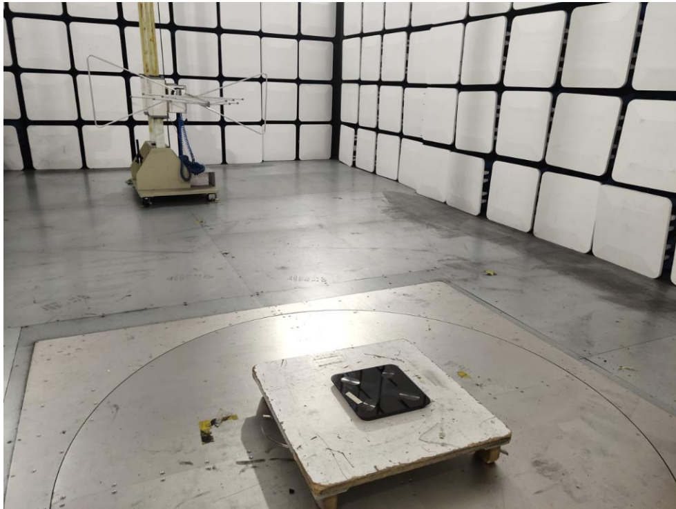
FCC ID: 2AQA6-H5010 Photo of Radiation Emission Test
