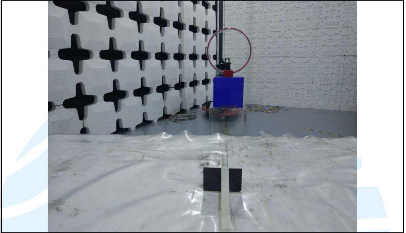
Radiated emission Test Setup (below 30 MHz)
