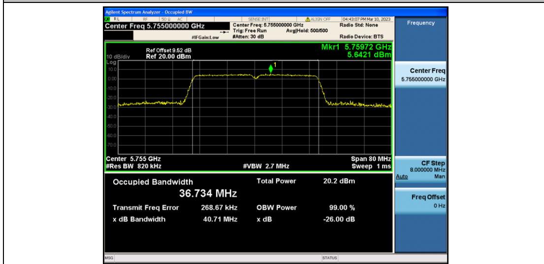
11N40SISO_Ant1_5755
