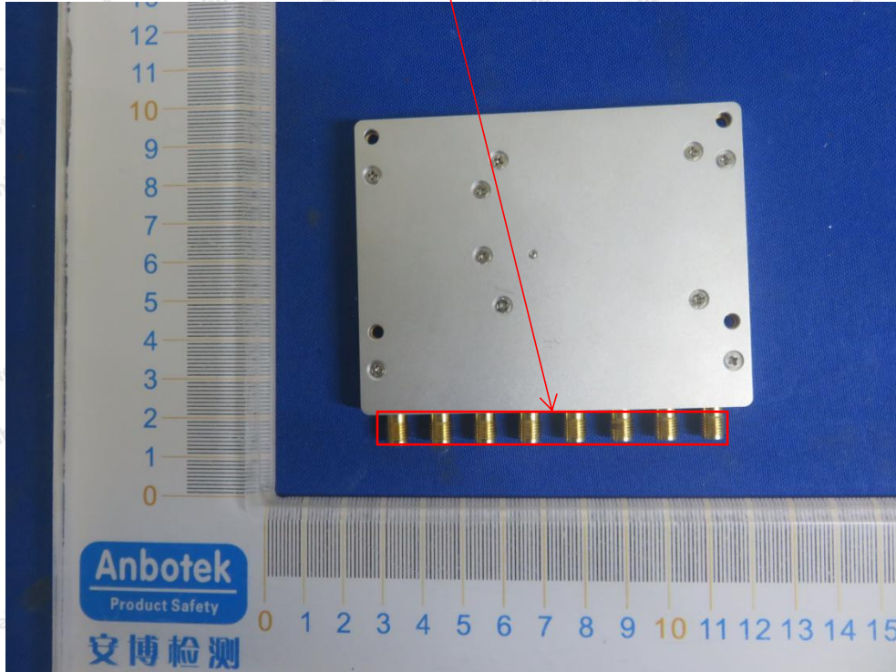
Ant Connector
