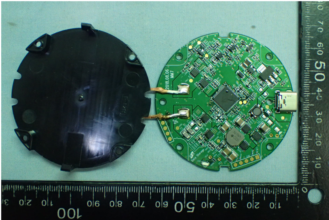
Figure 9 Internal View
