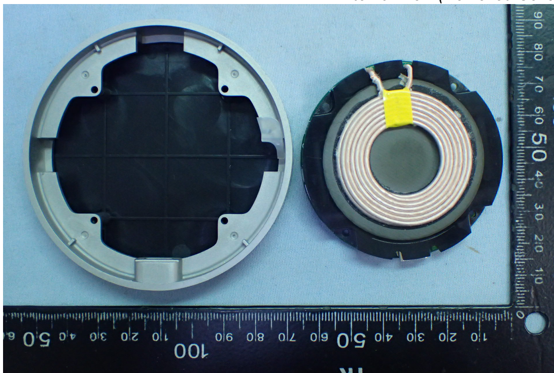
Figure 8 Internal View (Removed Cover)
