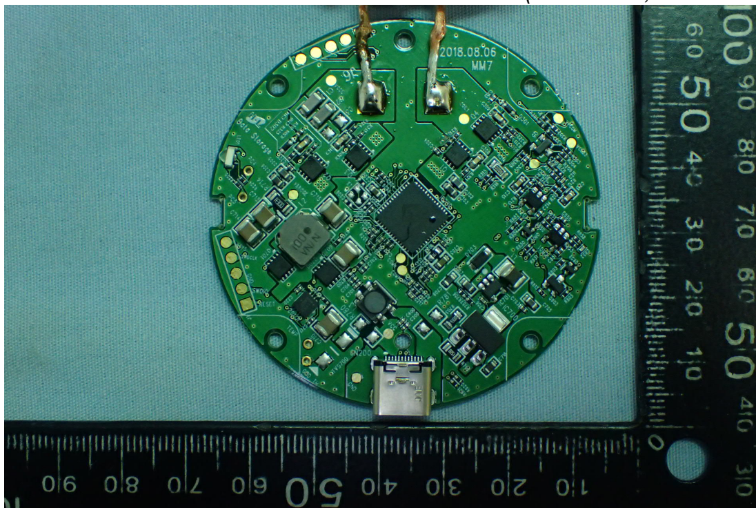
Figure 11 Internal View (Main Board, Front View)
