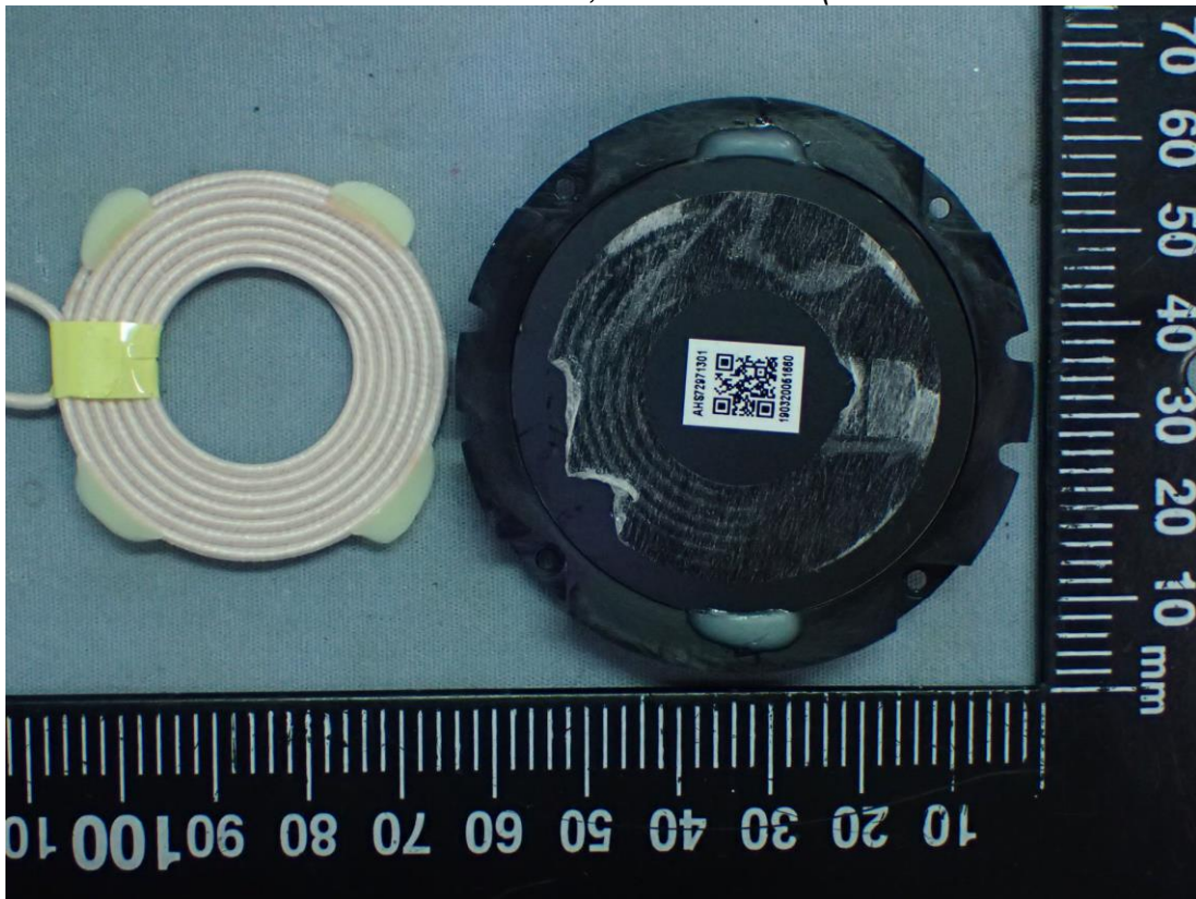
Figure 19 Model: HLW-TNMP7A, Internal View (Removed WPC Antenna)
