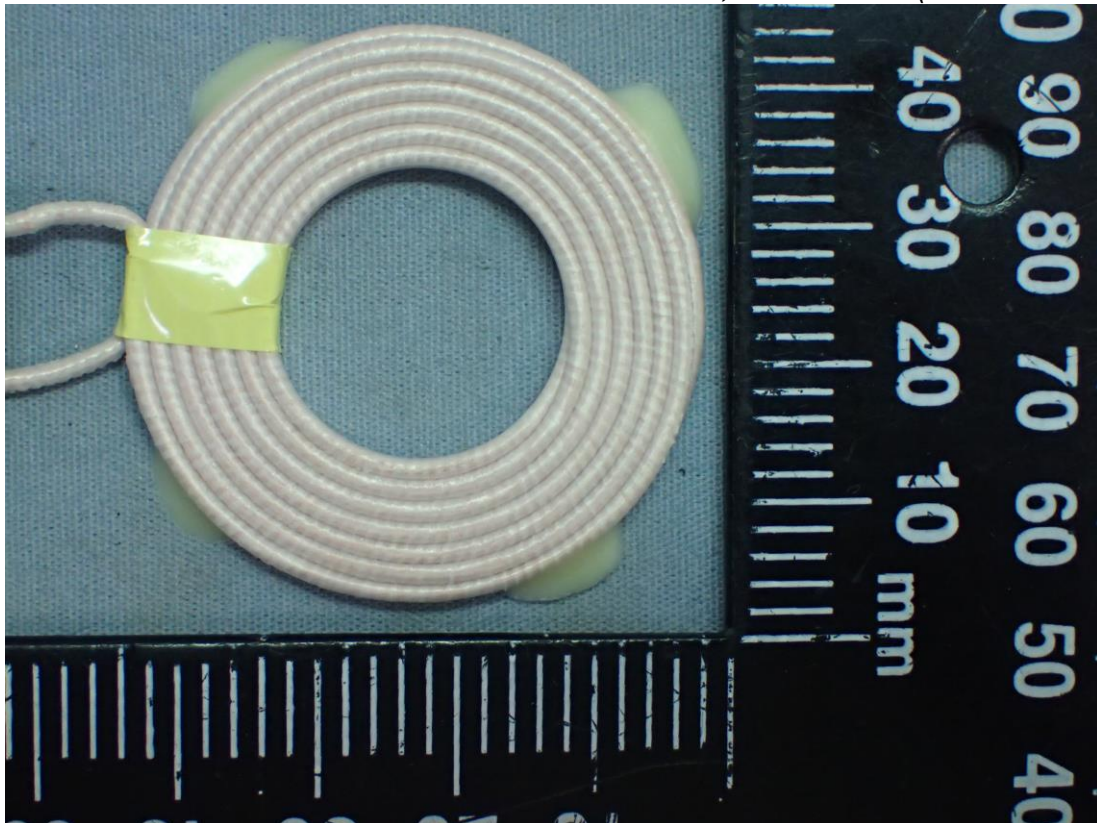
Figure 20 Model: HLW-TNMP7A, Internal View (WPC Antenna)
