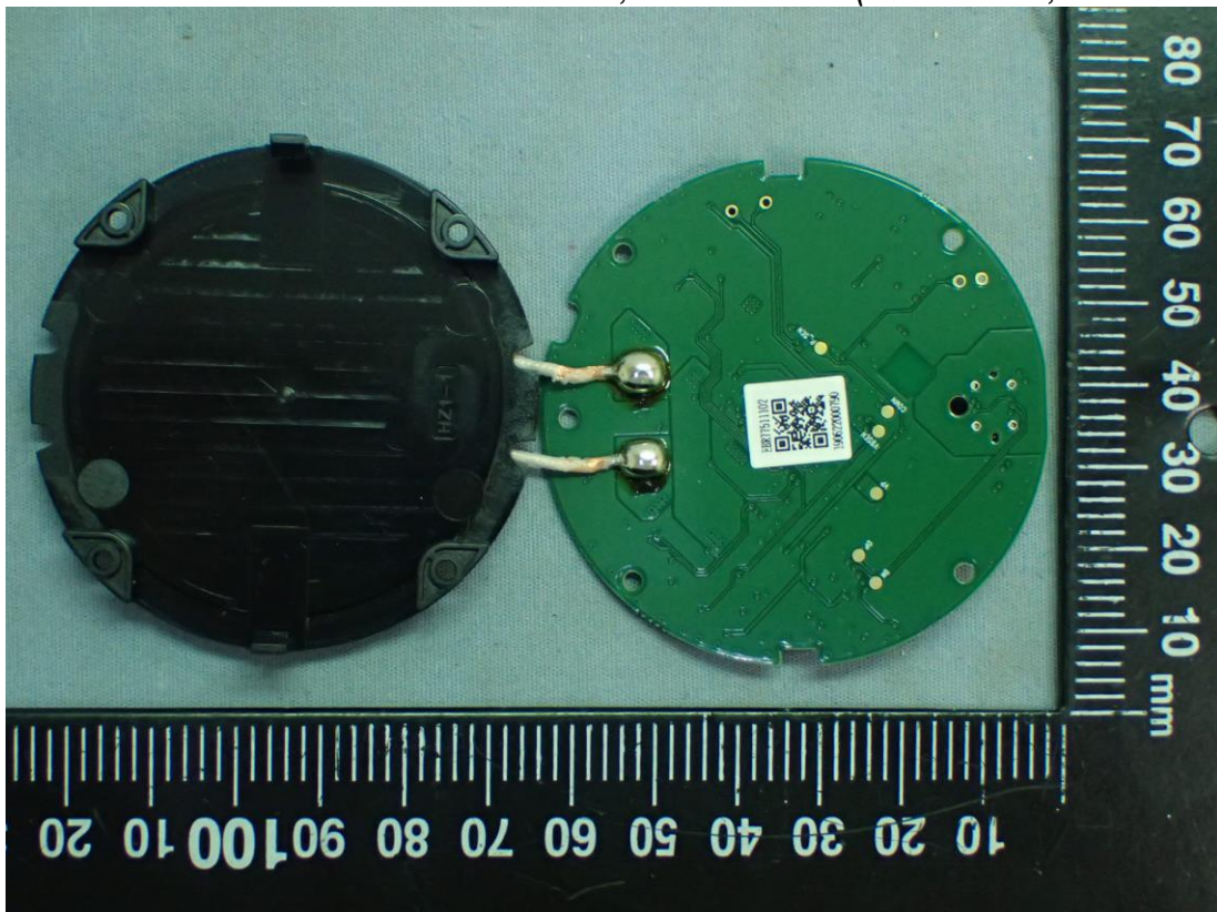
Model: HLW-TNMP7A, Internal View (Main Board, Back View)
