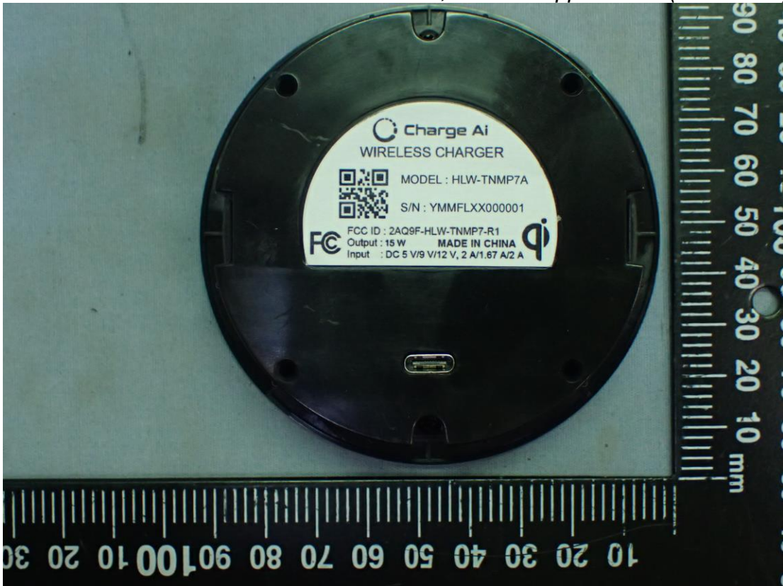
Model: HLW-TNMP7A, General Appearance (Back View)
