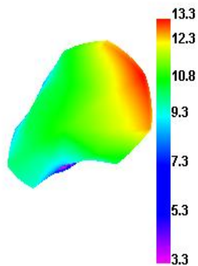
LTE5 20450 TRP
