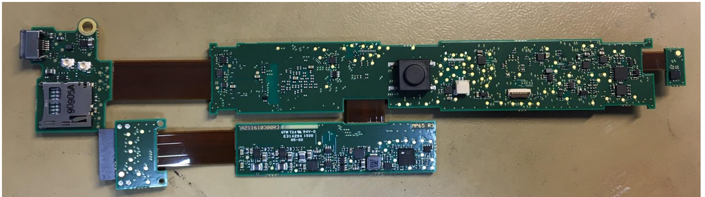
Mother board with radio module, front side
