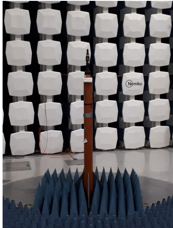
Radiated Emissions above 1 GHz
