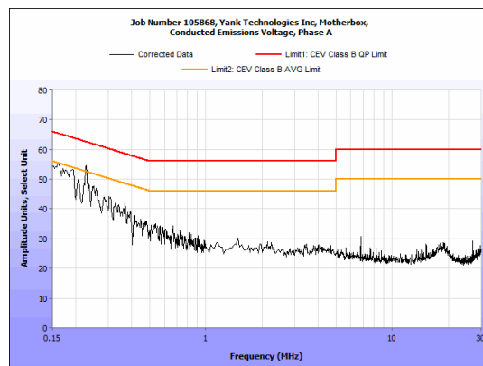
Figure 12: Conducted Emissions, phase, Dummy Load Terminated.
