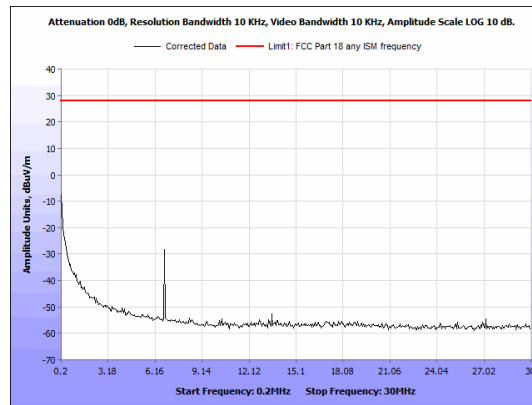
Figure 21: Radiated Emissions, 0.2-30 MHz, Perpendicular, standby
