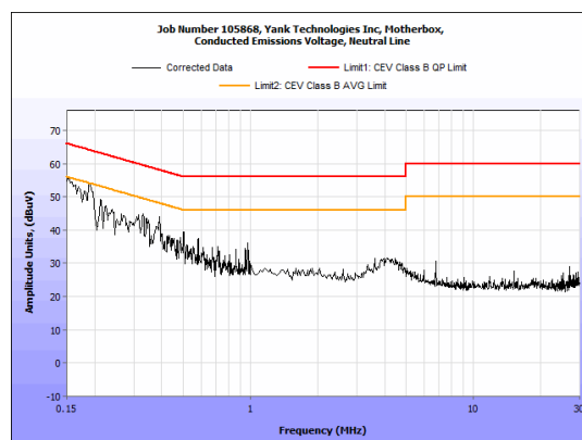
Figure 13: Conducted Emissions, neutral, Dummy Load Terminated.
