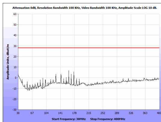
Figure 25: Radiated Emissions, 30-400 MHz, Vertical, standby
