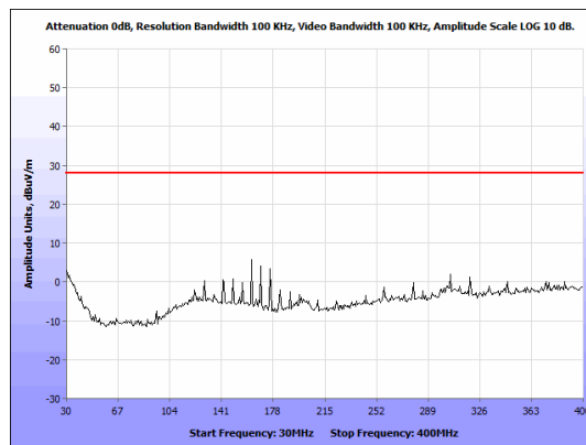
Figure 23: Radiated Emissions, 30-400 MHz, Horizontal, standby
