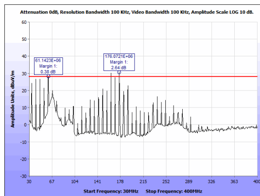
Figure 24: Radiated Emissions, 30-400 MHz, Vertical
