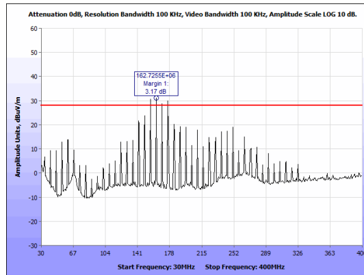
Figure 22: Radiated Emissions, 30-400 MHz, Horizontal
