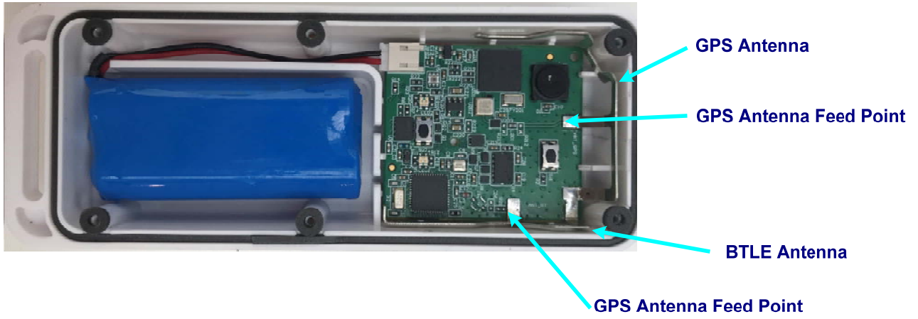
Figure 1 - Parsyl Trek - Internal View – PWB & Battery in Case
