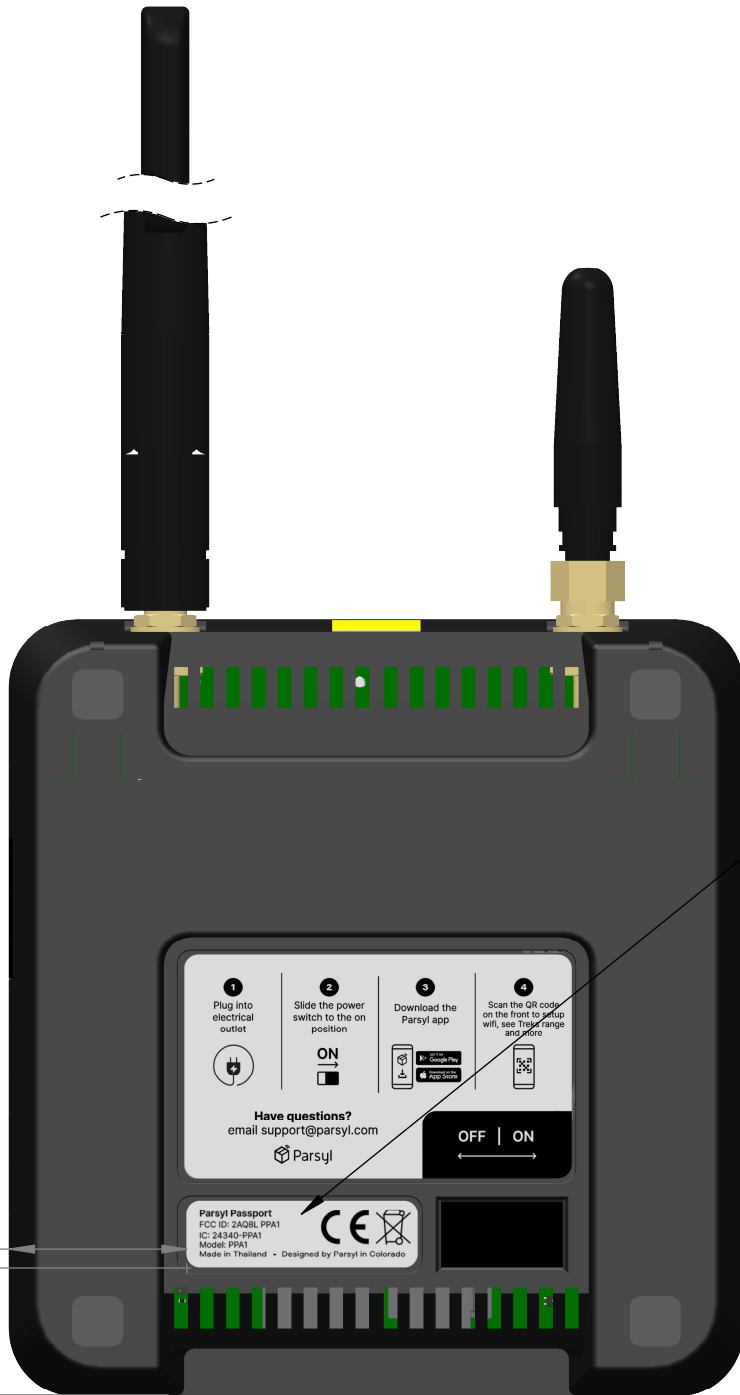
Parsyl Passport - back view antenna on the left only partially shown
