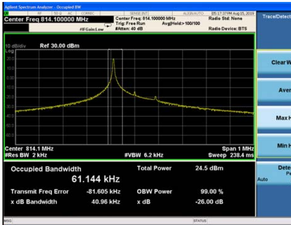
NB-IOT Band 26 BPSK 3.75kHz 1@0 CH-Middle
