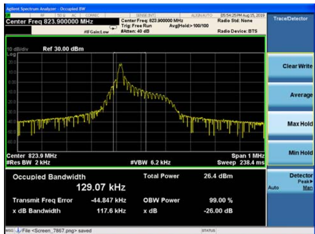
NB-IOT Band 26 BPSK 15kHz 1@0 CH-High
