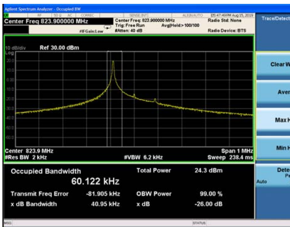
NB-IOT Band 26 BPSK 3.75kHz 1@0 CH-High
