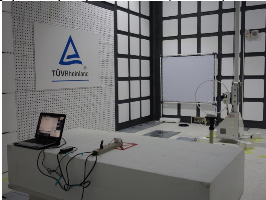
Photograph 5: Set-up for Spurious Emissions (Back View 4)
