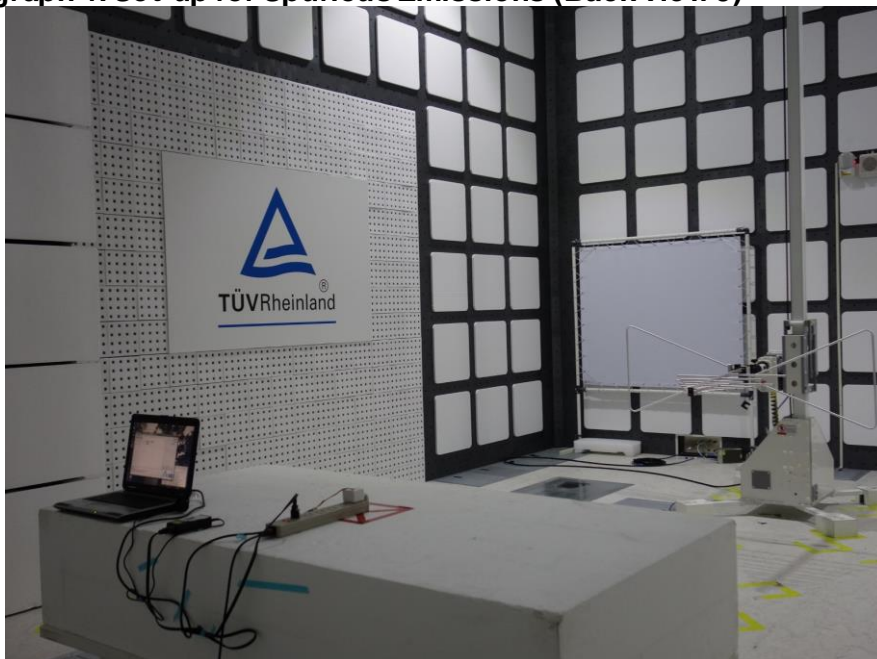
Photograph 4: Set-up for Spurious Emissions (Back View 3)
