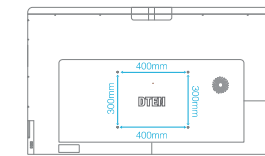
Mounting Hole Pattern: 400 x 300mm
