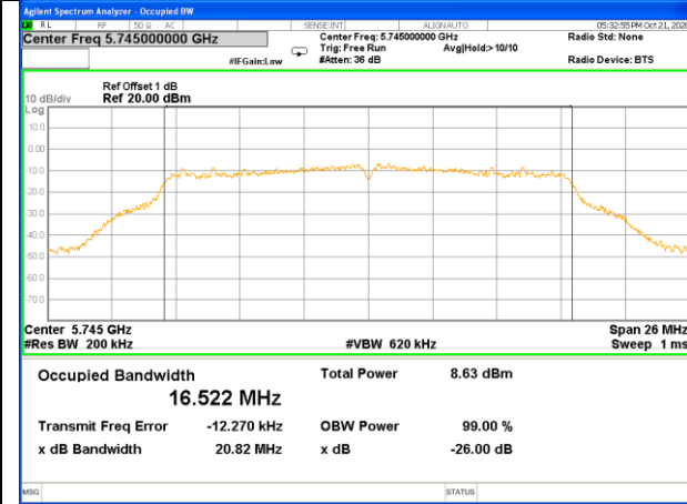
W58_11a20_Higher_26BW and 99%
