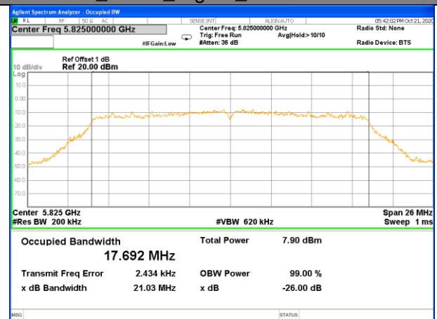
W58_11n20_Higher_26BW and 99%
