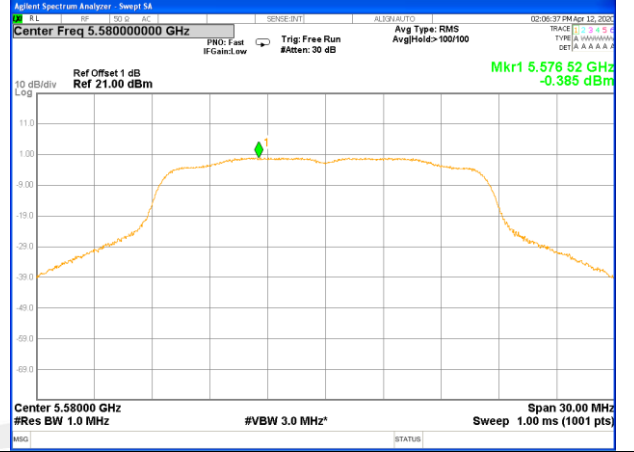
W56_11n20_Lower_Power Spectrum Density
