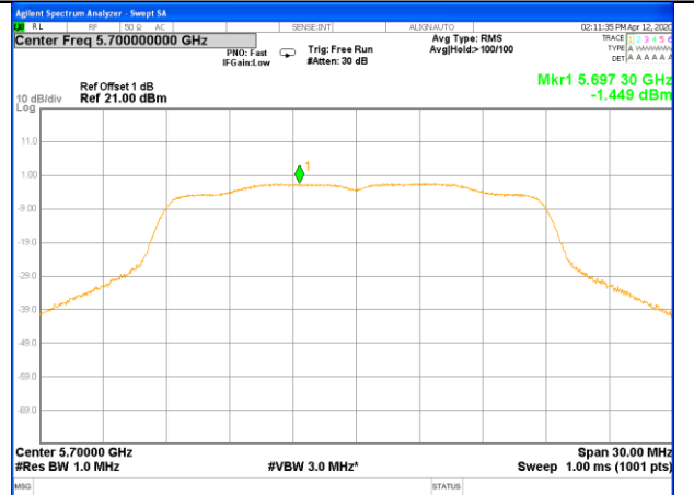
W56_11n20_Higher_Power Spectrum Density
