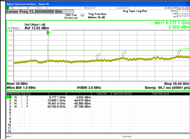
W52_11ac20_Higher_Conducted Spurious
