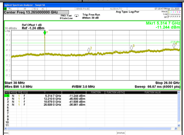
W53_11ac80_CH58(5290MHz)_Conducted Spurious
