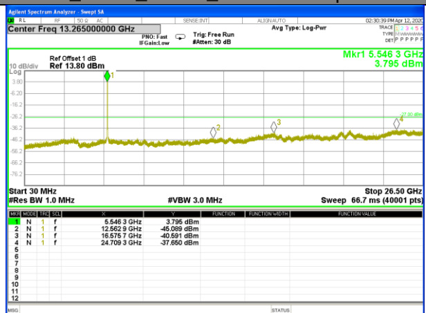
W56_11n40_Middle_Conducted Spurious
