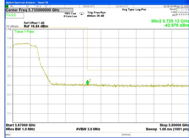
W56_11ac80_Higher_Conducted Spurious
