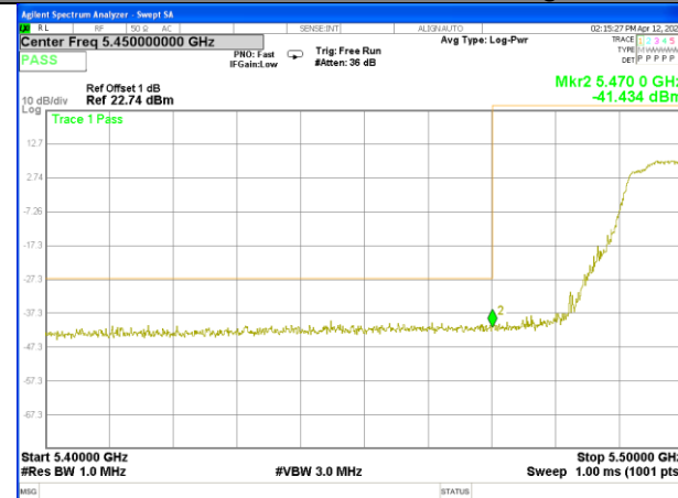
W56_11n40_Lower_Conducted Spurious
