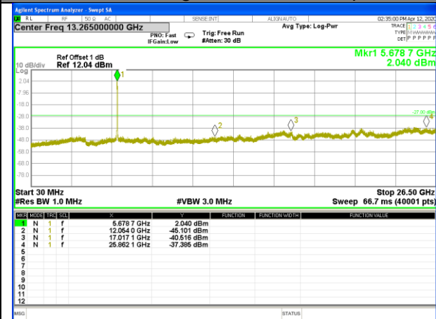
W56_11ac40_Higher_Conducted Spurious
