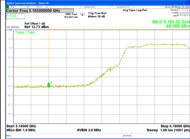
W52_11ac20_Lower_Conducted Spurious
