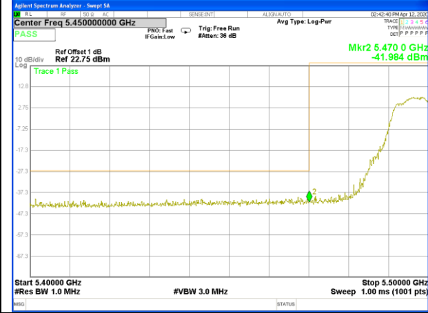
W56_11ac40_Lower_Conducted Spurious
