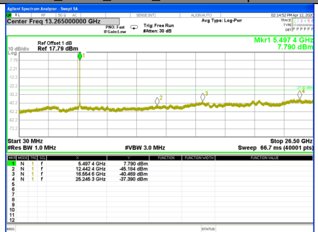
W56_11n20_Lower_Conducted Spurious
