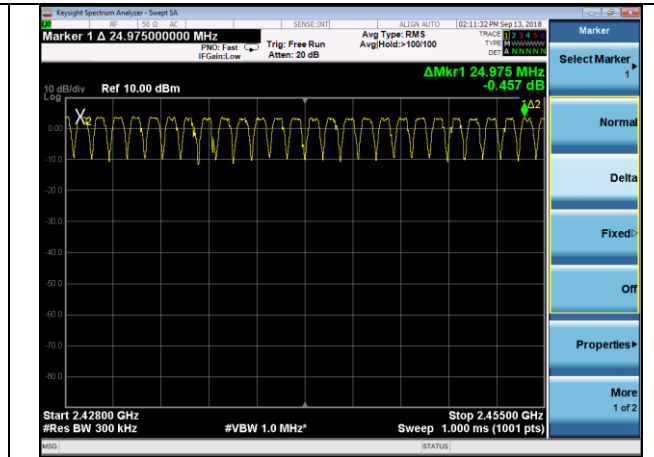
GFSK Modulation
