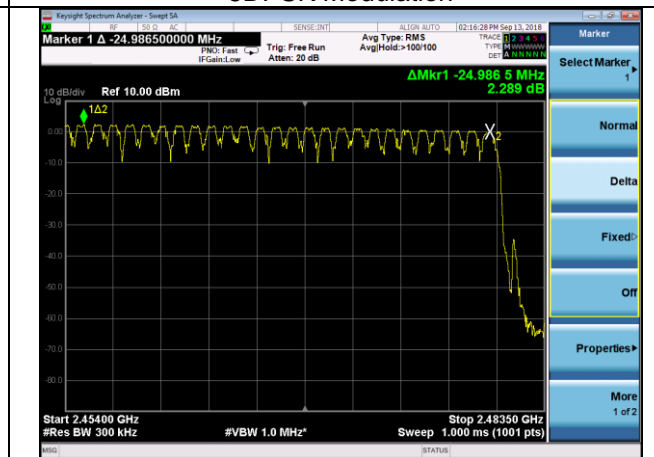
8DPSK Modulation
