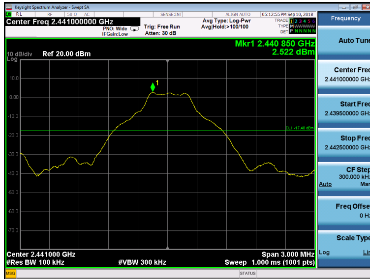
Channel 39
