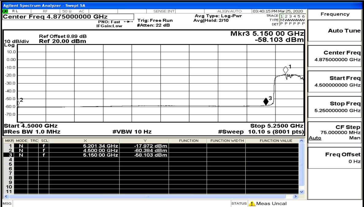
IEEE 802.11ac80 / Channel 42 / 5210MHz / Average
