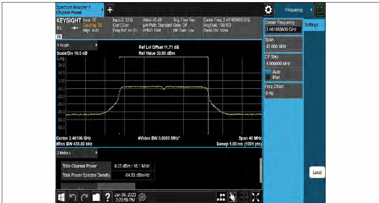
11N20SISO-Ant1-2462-----7.81-94.63-0.24
