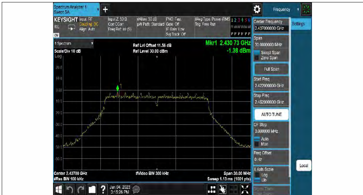
11G-Ant1-2437-0~Reference--1.38
