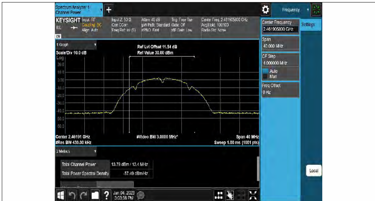
11B-Ant1-2462-----13.72-98.33-0.07
