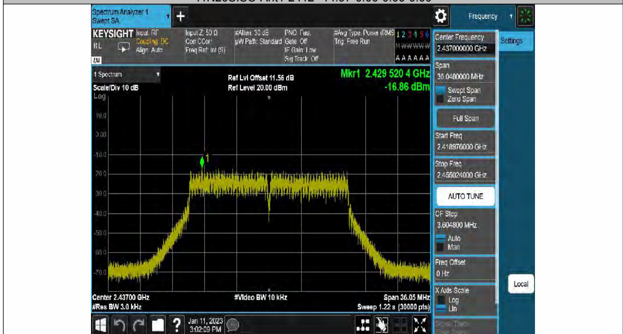
11N20SISO-Ant1-2437--16.86-0.00-0.00-0.00
