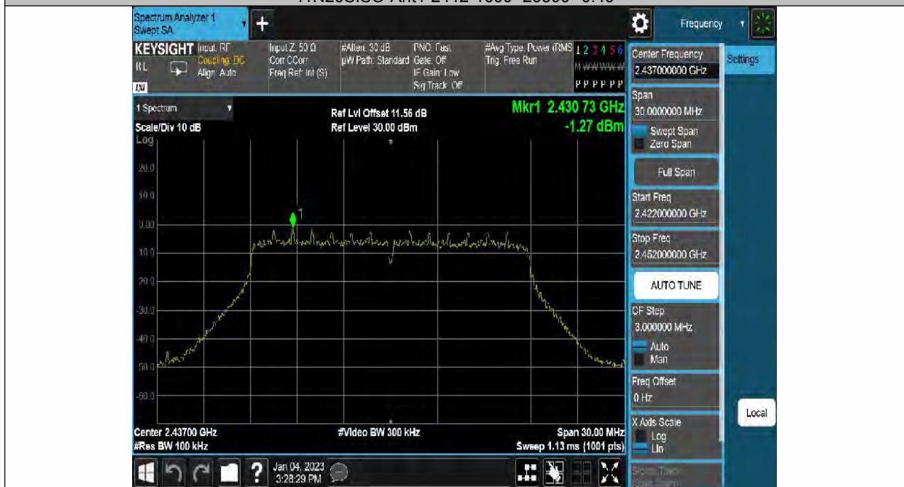
11N20SISO-Ant1-2437-0~Reference--1.27
