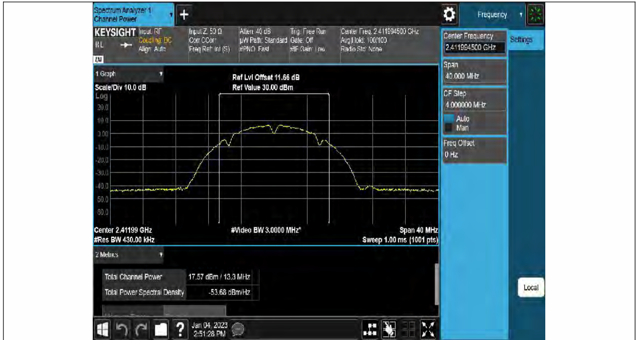
11B-Ant1-2412-----17.53-98.99-0.04
