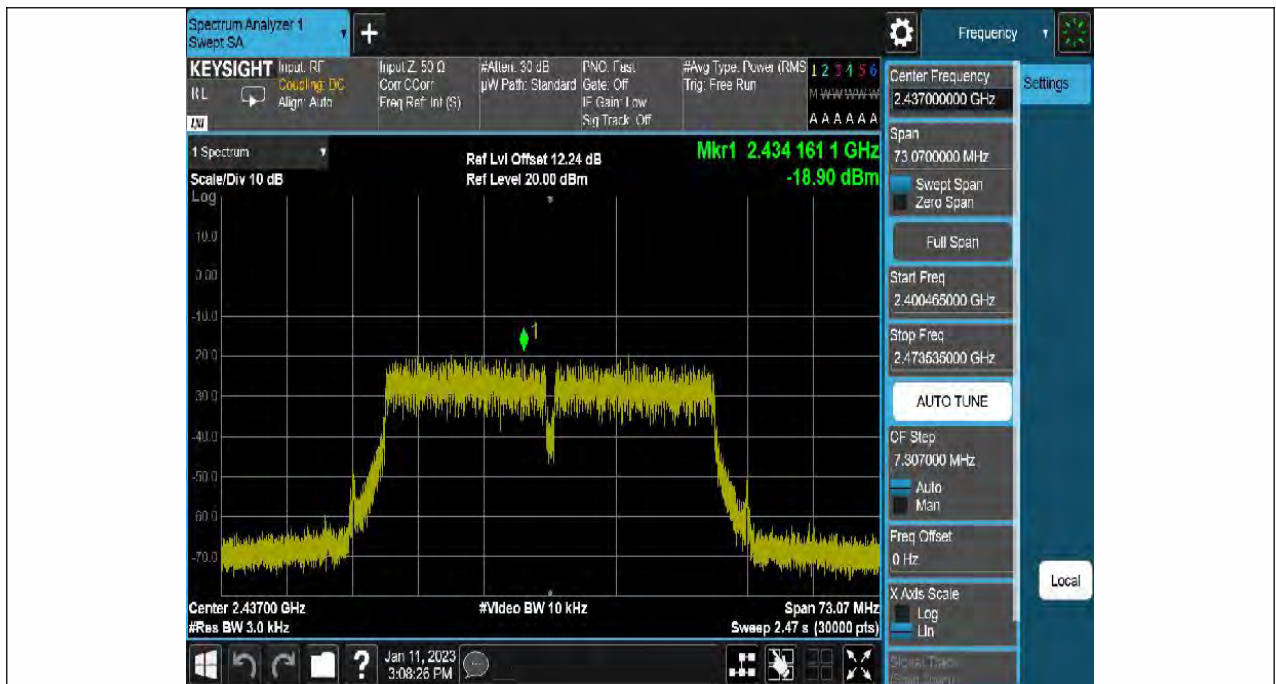
11N40SISO-Ant1-2437--19.58-0.68-0.00-0.00
