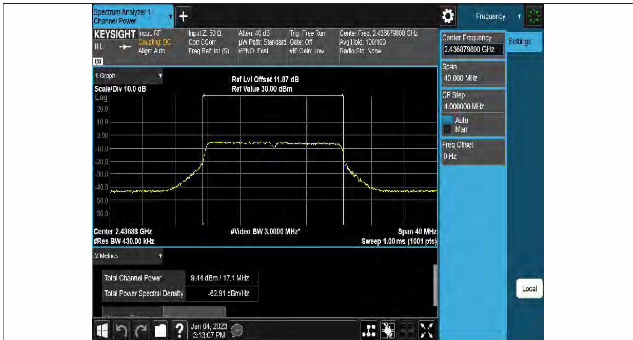
11G-Ant1-2437-----9.13-93.19-0.31
