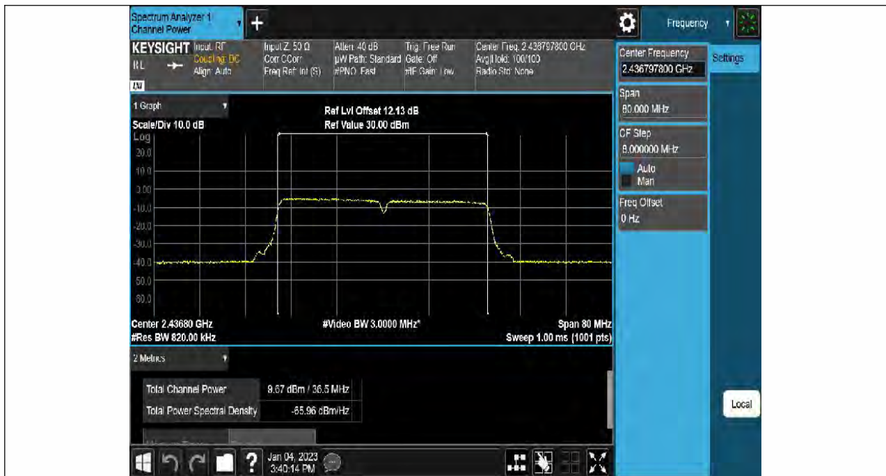
11N40SISO-Ant1-2437-----9.10-87.68-0.57
