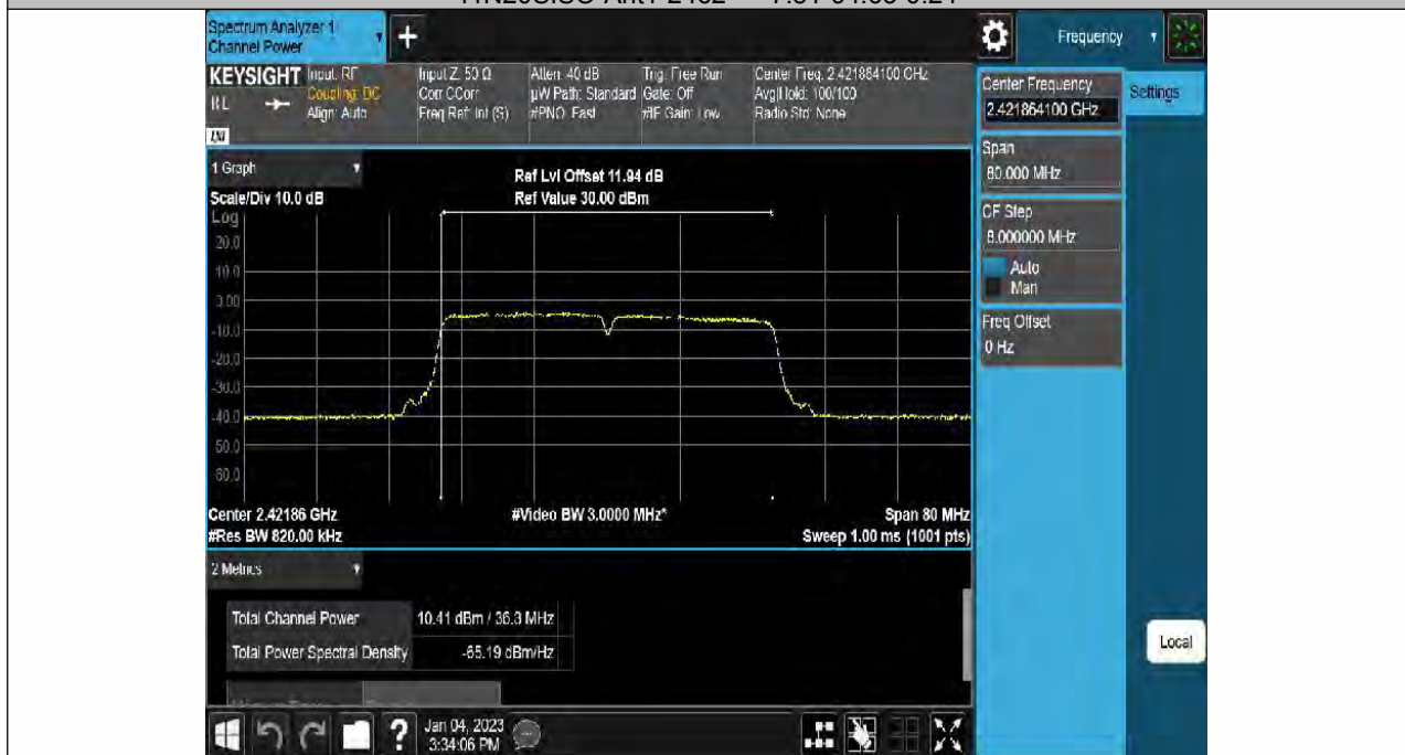
11N40SISO-Ant1-2422-----10.03-91.52-0.38
