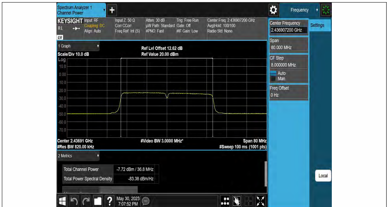
11N40SISO-Ant1-2437-----9.10-87.68-0.57
