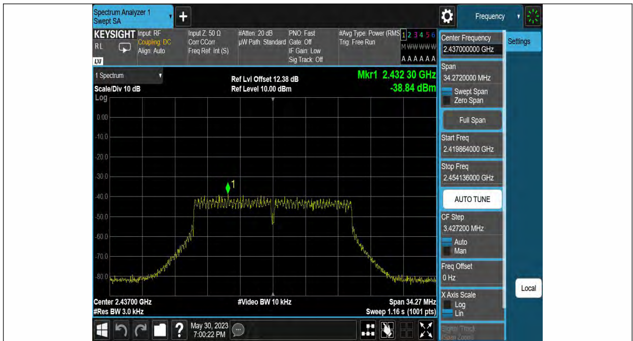
11G-Ant1-2437--17.02-0.00-0.00-0.00
