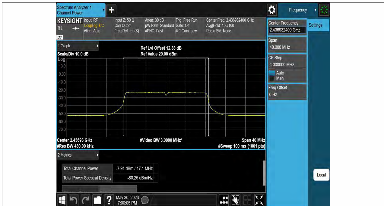
11G-Ant1-2437-----9.13-93.19-0.31
