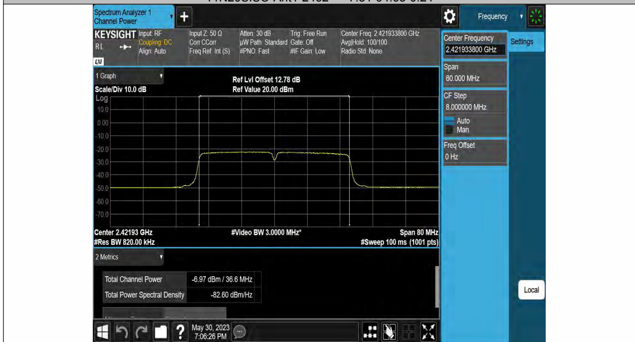
11N40SISO-Ant1-2422-----10.03-91.52-0.38
