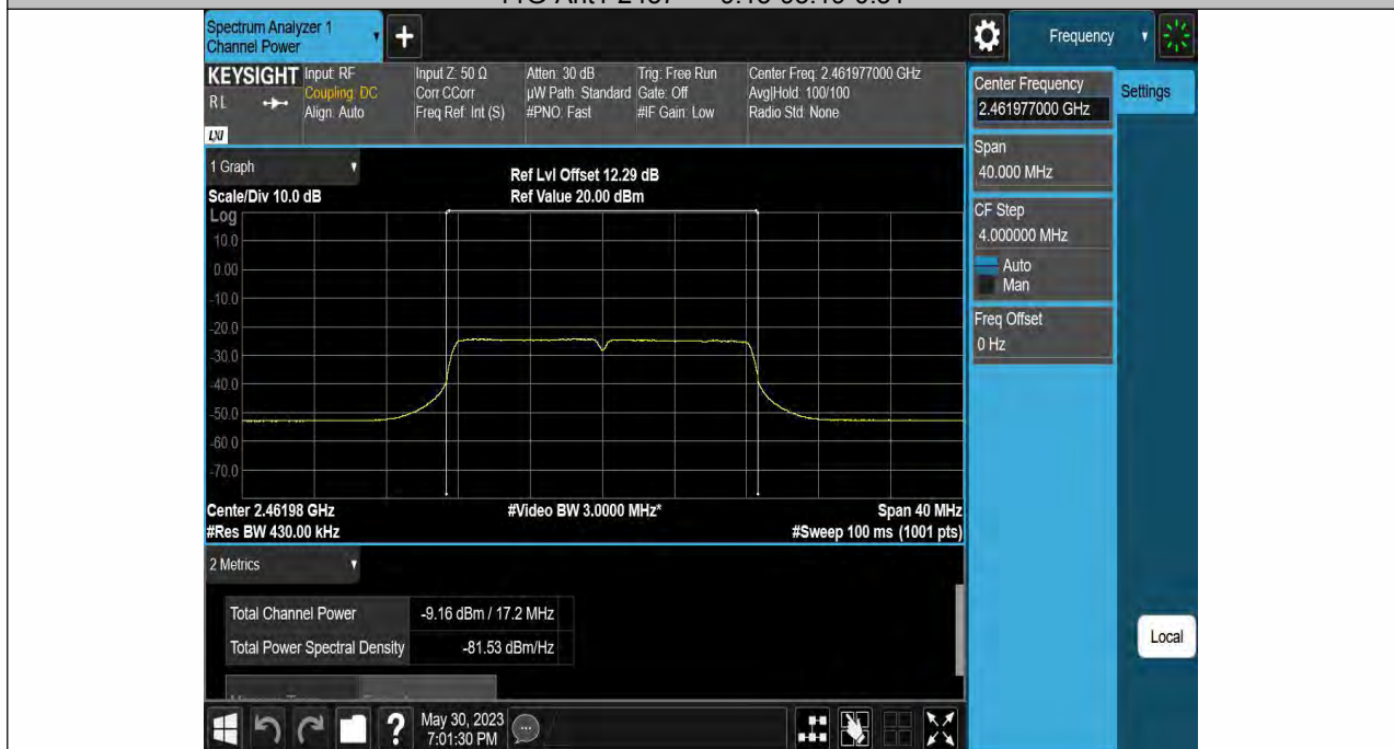
11G-Ant1-2462-----7.84-92.08-0.36
