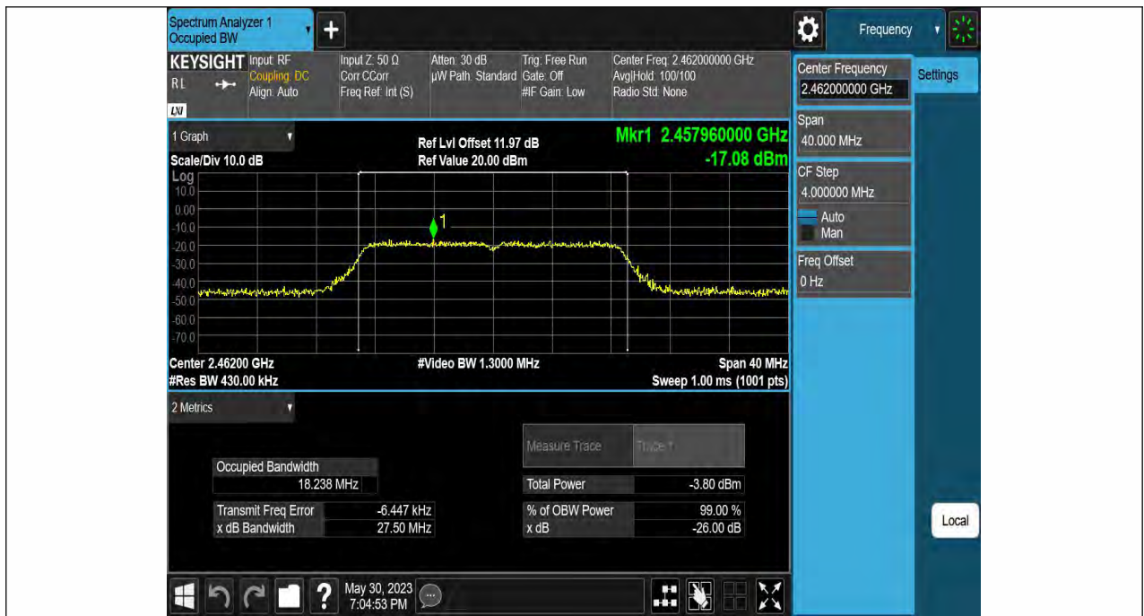
11N20SISO-Ant1-2462
