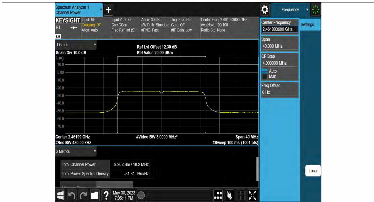
11N20SISO-Ant1-2462-----7.81-94.63-0.24
