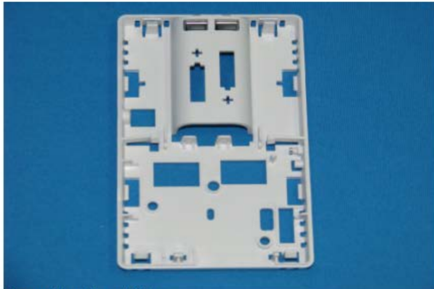
Bottom Cover Internal View
