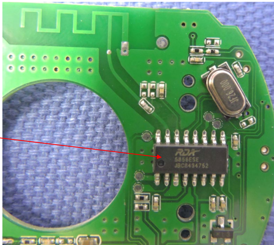
RF chip
