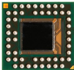
Bottom view of A121 package substrate with on-chip Integrated Circuit included
