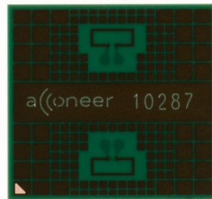
Top view of A121 package substrate with integrated antennas
