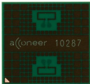
Top view of A111 package substrate with integrated antennas
