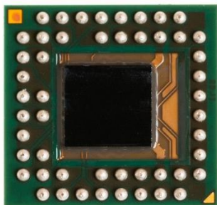
Bottom view of A111 package substrate with on-chip Integrated Circuit included
