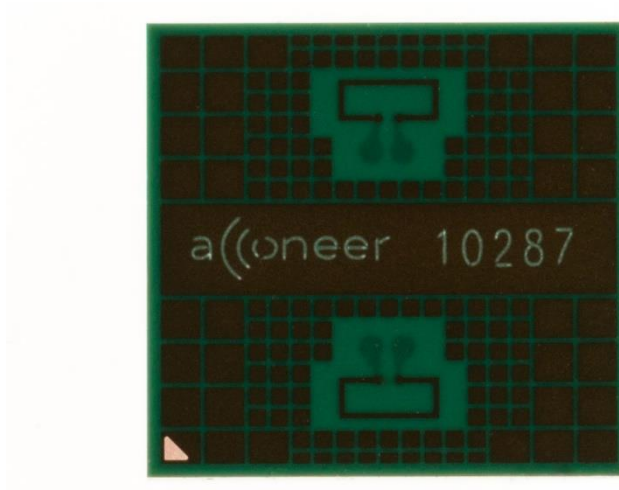
Figure 1, Frontside of the A111 sensor.
