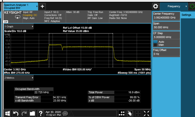
26dB Bandwidth Spectrum Plot of Worst Value 5MHz+20MHz / QPSK
