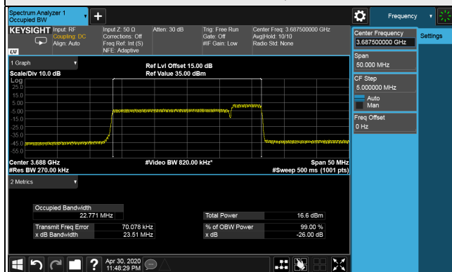
99% Occupied Bandwidth Spectrum Plot of Worst Value 20MHz+5MHz / QPSK
