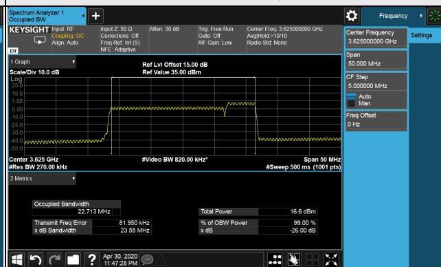
26dB Bandwidth Spectrum Plot of Worst Value 20MHz+5MHz / QPSK
