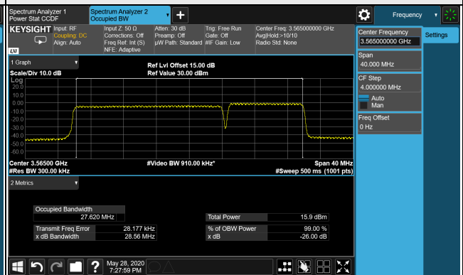
26dB Bandwidth Spectrum Plot of Worst Value 20MHz+10MHz / 16QAM
