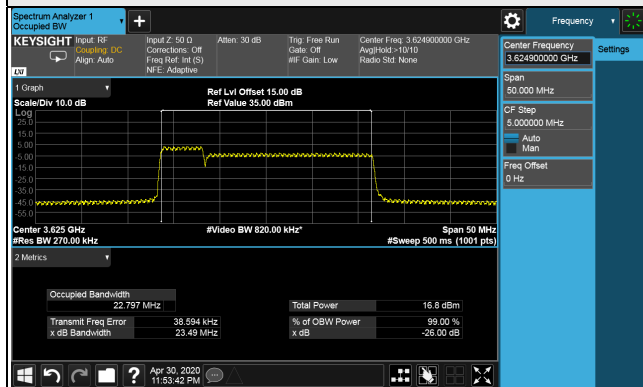
99% Occupied Bandwidth Spectrum Plot of Worst Value 5MHz+20MHz / QPSK
